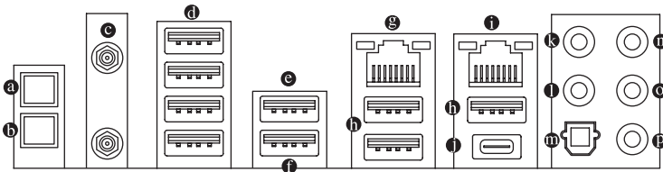
Back View-A
